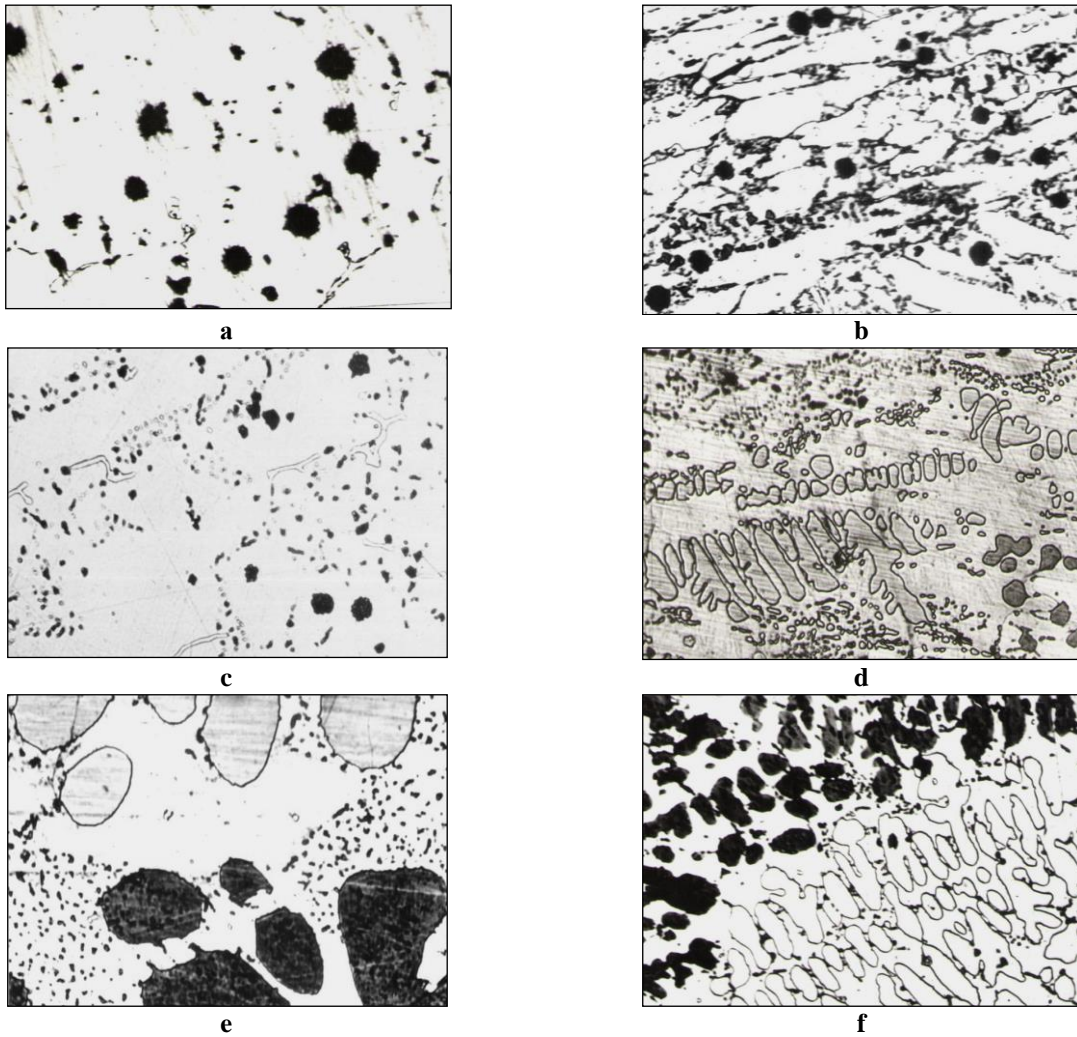
Fig. 4. Microstructure (x300) Fe – 9.1 % B – 1.45 % C (a, b); Fe – 12.3 % B – 0.82 % C (c, d); Fe – 14.3 % B – 0.8 % C (e, f) alloys: a, c, e – V_{cool} = 10 K/s; b, d, f – V_{cool} = 10^3 K/s.
