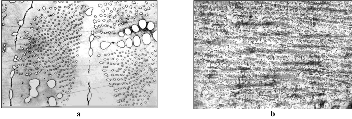
Fig. 3. Microstructure of Fe – 10.8 % B – 0.3 % C alloy (x300): a – V_{cool} = 10 K/s; b – V_{cool} = 700 K/s
