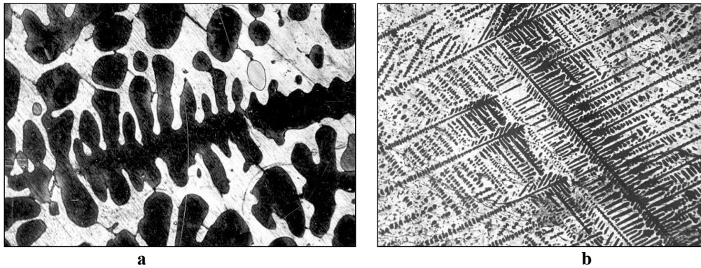
Fig. 1. Microstructure of Fe – 12.1 % B – 0.1 % C alloy (x300): a – V_{cool} = 10 K/s; b – V_{cool} = 10^3 K/s
