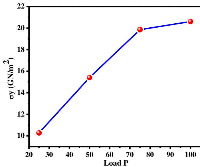
Fig. 10. Load (P) dependent yield strength (σ y ).
